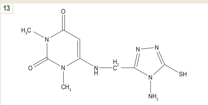
Fig. 13. 6-(((4-amino-5-mercapto-4H-1,2,4-triazole-3-yl)methyl)amino)-1,3-dimethylpyrimidine-2,4(1H,3H)-dione.
