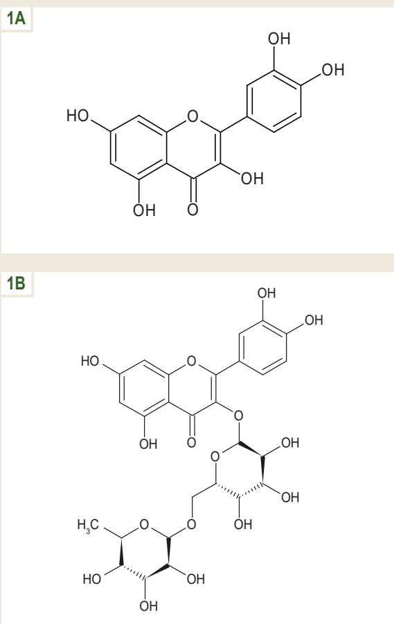
Fig. 1. Chemical structure of quercetin (A) and rutin (B).
