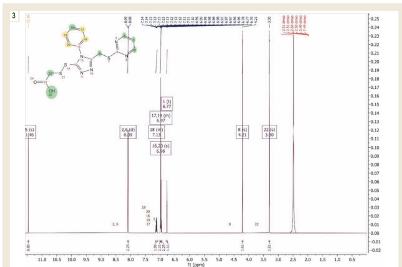
Fig. 3. ^1\text{H} NMR spectrum 2-((5-((2,6-dioxo-1,2,3,6-tetrahydropyrimidin-4-yl)-4-phenyl-4H-1,2,4-triazol-3-yl)disulfaneyl)acetic acid ( 4a ).
